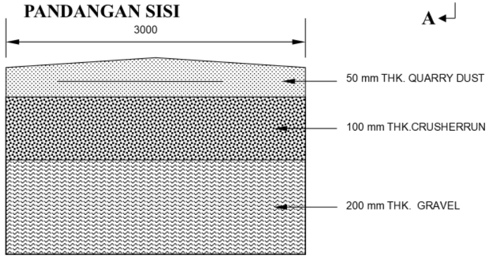
KERATAN A - A
